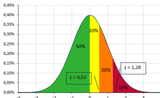
Chart 4.4: Probability density of a standard normal distribution around 0 x: z-score / y: density
