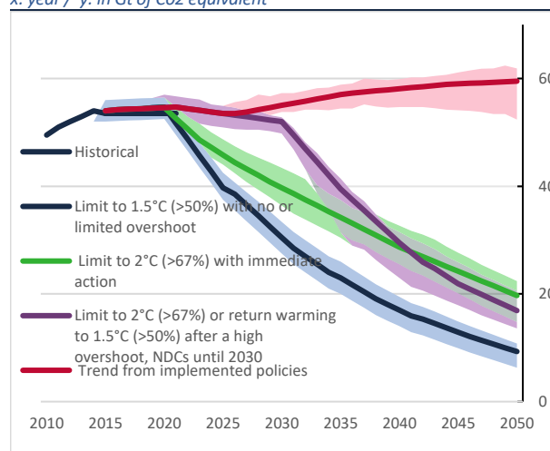
Chart 1.62: GHG emissions reductions according to different trajectories x: year / y: in Gt of CO 2 equivalent
